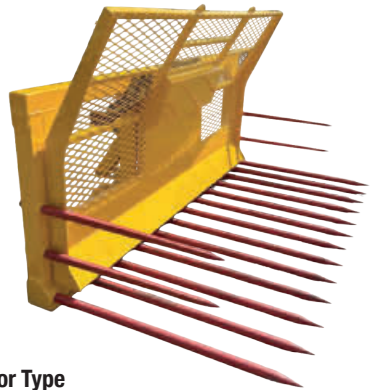
9' Push Off HD Buckrake - Tractor Type
