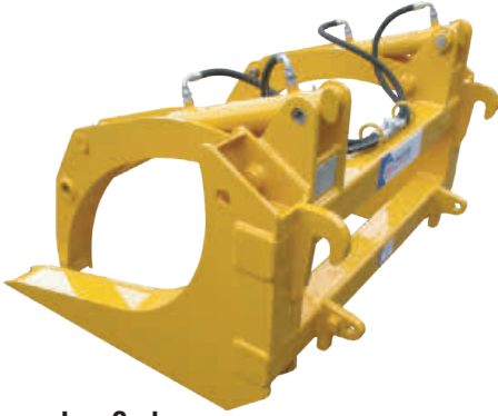
Log Grab
